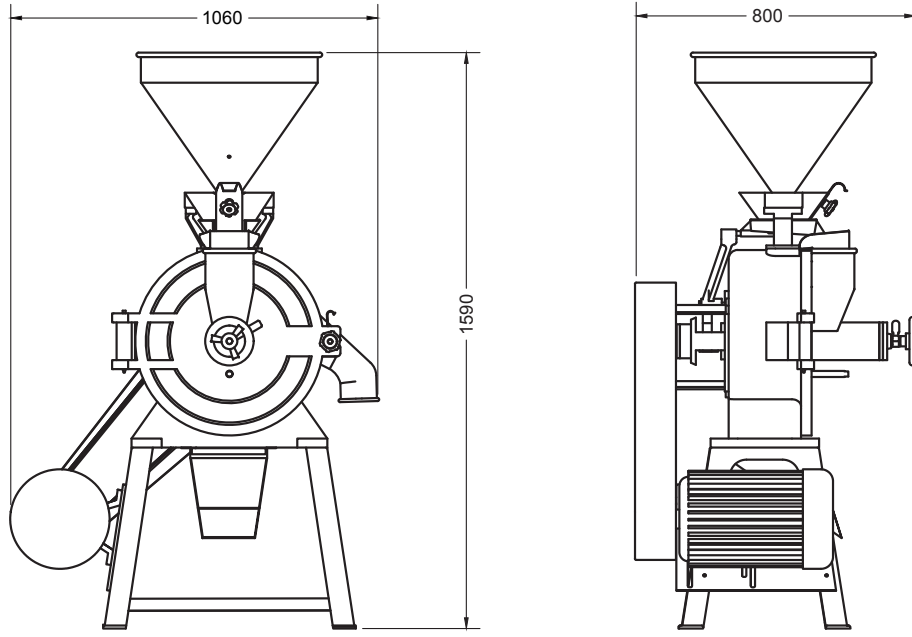
TKS 40-TD
