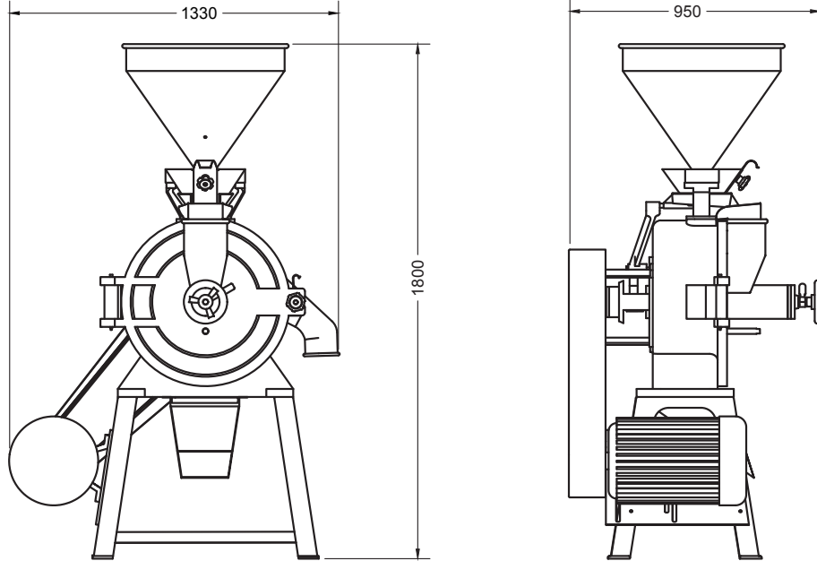
TKS 50-TD
